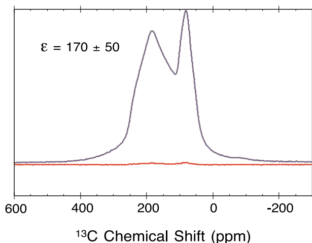
Fig. 2. DNP CP spectra of static 1\text{-}^{13}\text{C} -glycine (0.39 M) dispersed in a 60:40 water/glycerol solution containing 80 mM 4-amino TEMPO. The spectra were recorded at 20 K with (upper trace) and without (lower trace) microwave irradiation. A ^1\text{H} DNP enhancement of 170 \pm 50 was observed with \sim 1.0\text{ W} of microwave power incident on the sample. Eight transients were recorded. The peak at \sim 75 ppm arises from glycerol at natural abundance.
