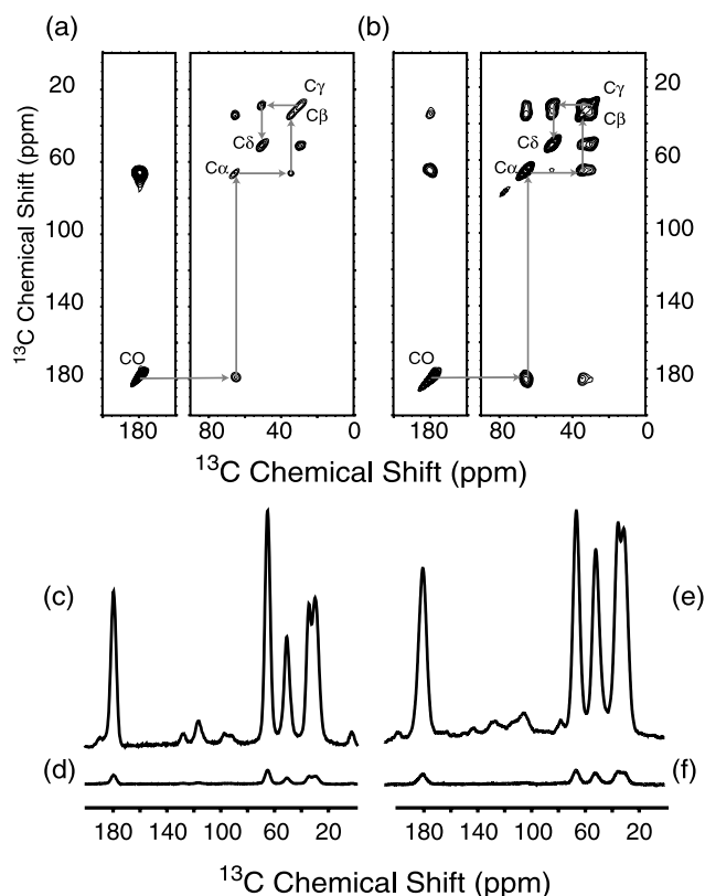
Fig. 5. Two-dimensional ^{13}\text{C} - ^{13}\text{C} correlation spectra of \text{U-}^{13}\text{C} , ^{15}\text{N} proline. In (a), the SPC5 dipolar recoupling sequence was applied during a double quantum mixing period. The MAS frequency was 6 kHz, the mixing time was 1.33 ms, and the temperature was regulated at 97 \pm 0.8 K. In (b), correlations were established by proton-driven spin diffusion for a mixing time of 10 ms. The MAS frequency was 7 kHz, and the temperature was unregulated but remained within the range 98–101 K. In both cases, 16 transients were acquired for each of 128 increments in the t_1 dimension, and the DNP enhancement was approximately 17. In (c) and (d), we show one dimensional ^{13}\text{C} MAS spectra obtained with and without DNP, respectively, using SPC5 recoupling with a double quantum phase cycle; (e) and (f) are CP spectra with and without DNP. The apparent intensity differences between the spectra in (c) and (e) are due to recoupling dynamics at short excitation times [31].
