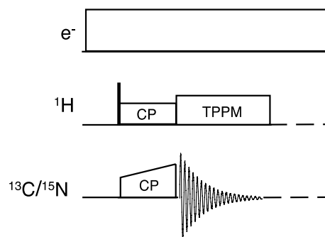
Fig. 1. Cross-polarization with continuous microwave irradiation. In all cases, the electron resonance offset was set to maximize the ^1\text{H} enhancement.
